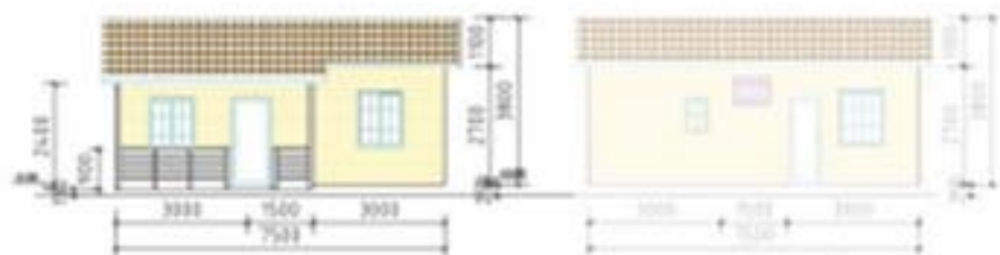
Back Elevation
