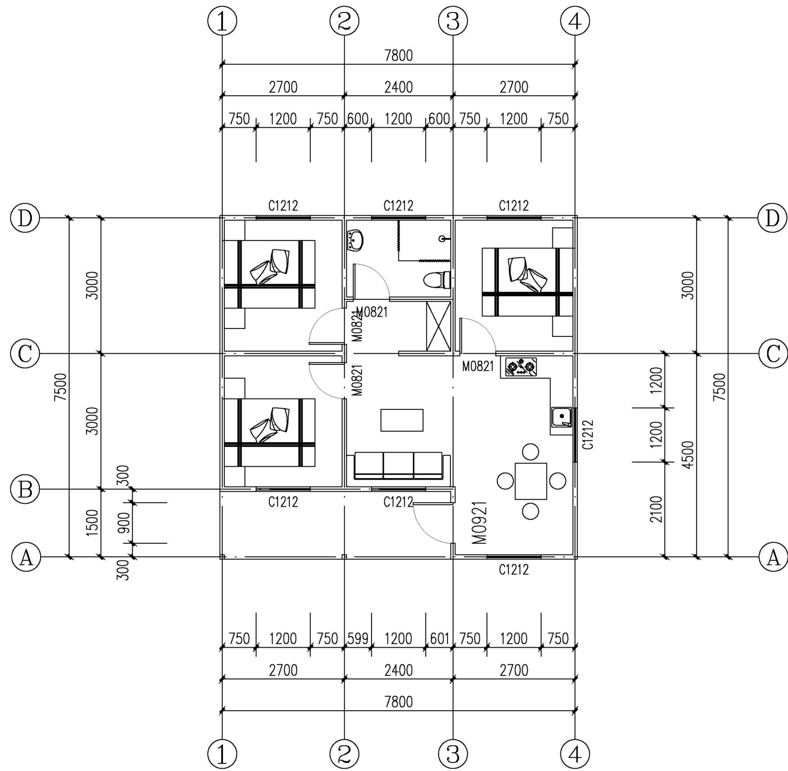
Plan View 1:100
