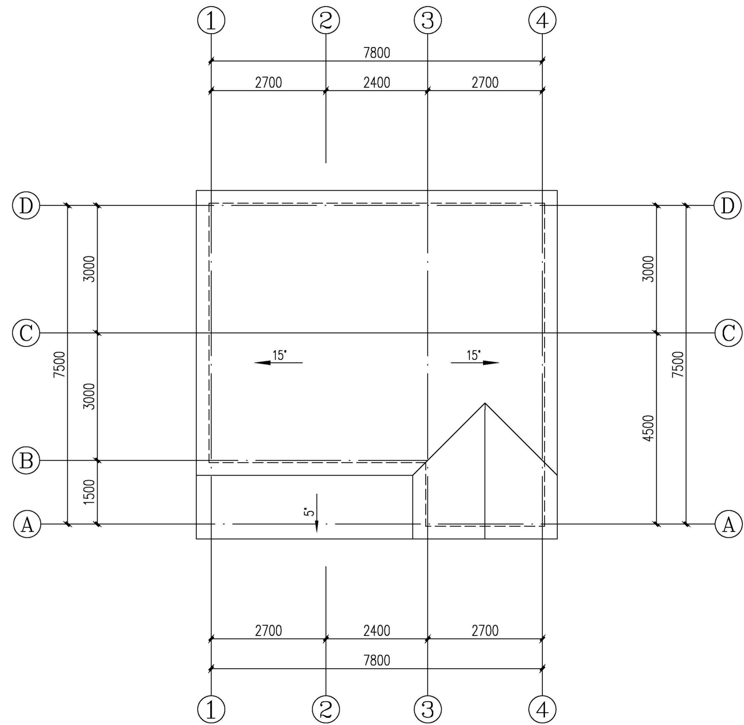
Roof Plan View 1:100
