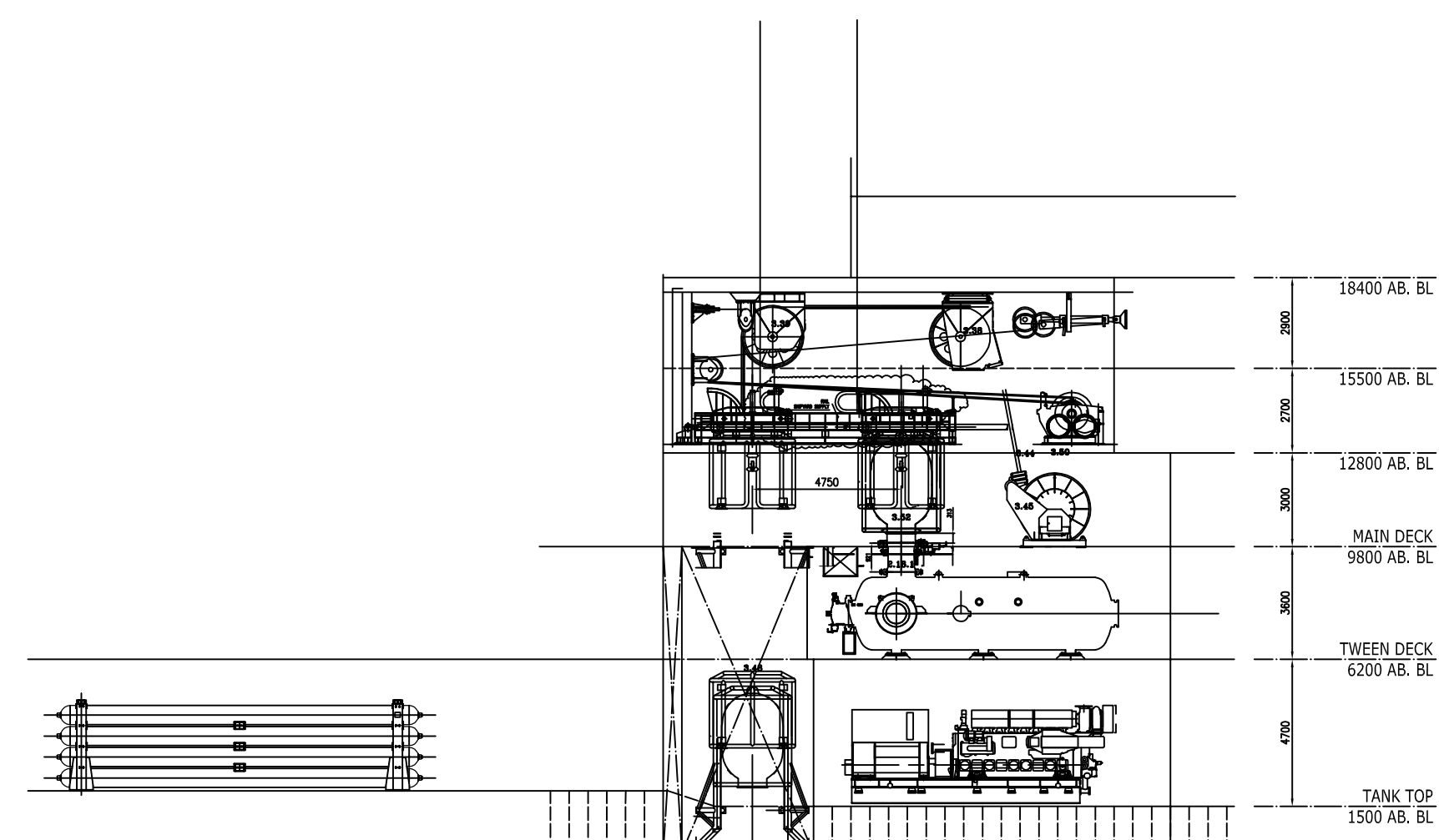
SECTION THROUGH CENTER OF MOONPOOL
