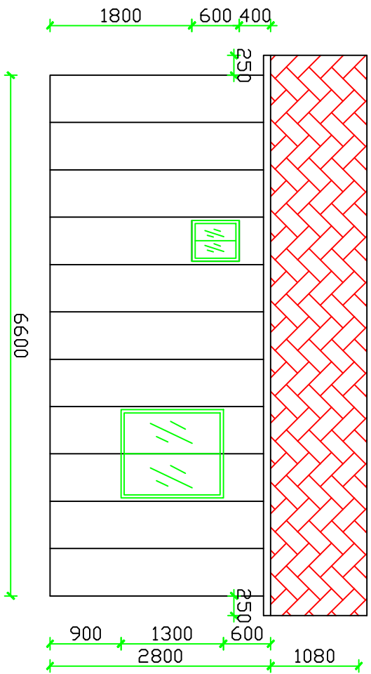
Rear Elevation
