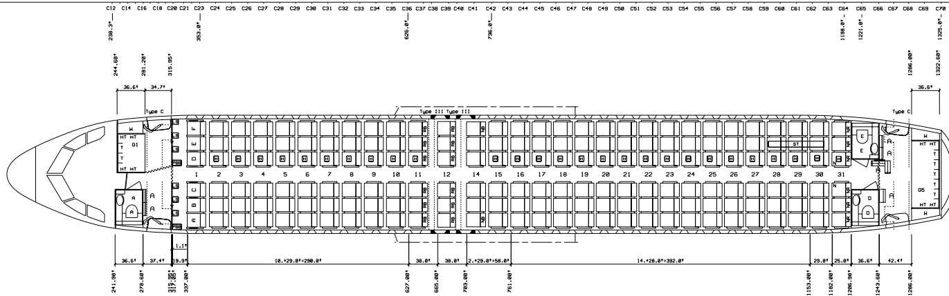
6 ABREAST CONSTANT SECTION
