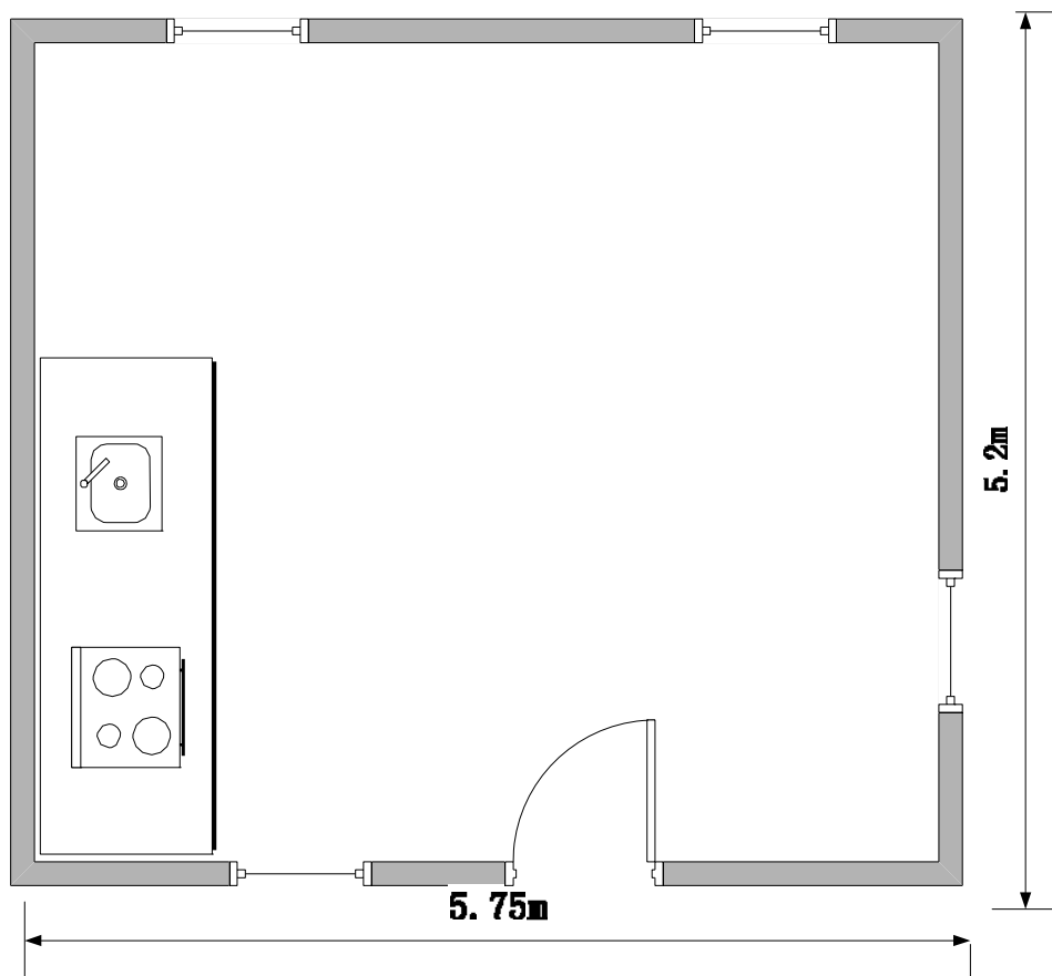
5.2*5.75*2.5/3.3m---30m 2 house drawing
