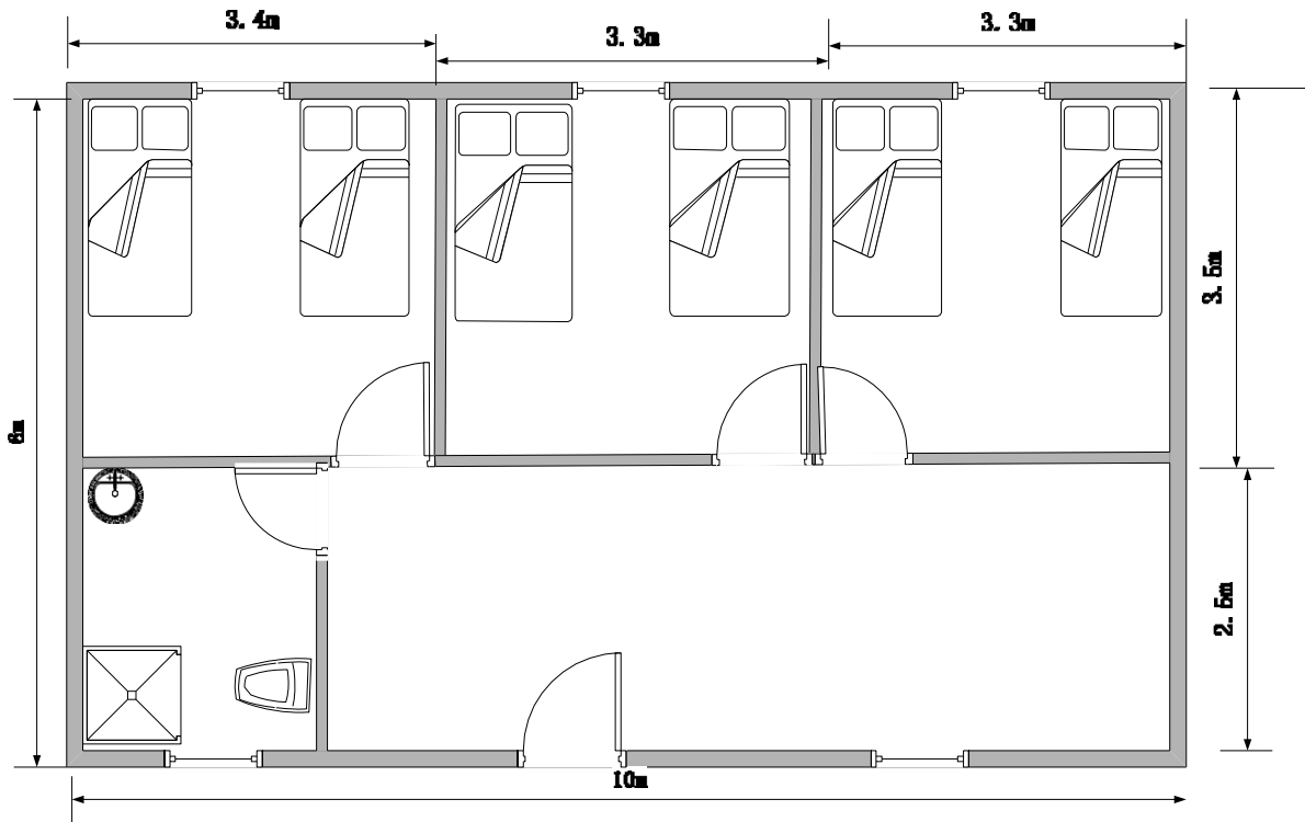
10*6*2.5/3.3m---60m2 house drawing
