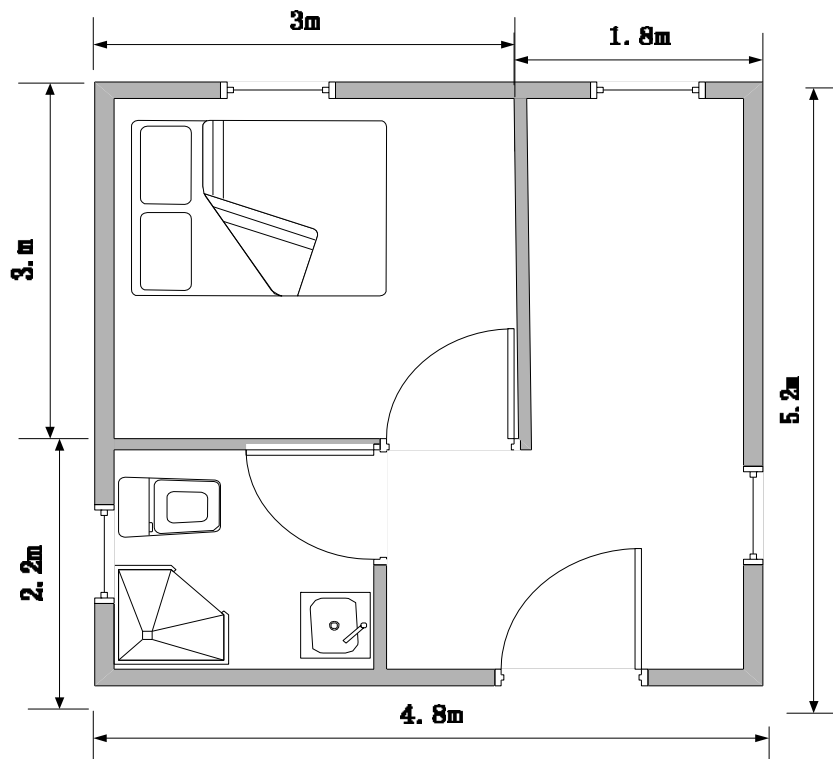
5.2*4.8*2.5/3.3m---30m 2 house drawing
