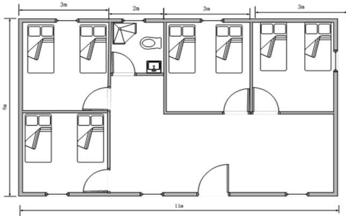
11*6*2.5/3.3m---66m2 house drawing
