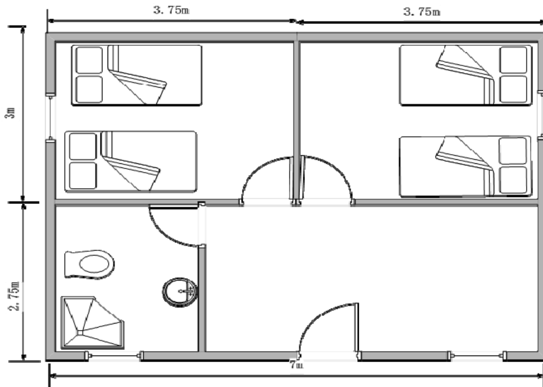
7*5.75*2.5/3.3m---40m2 house drawing
