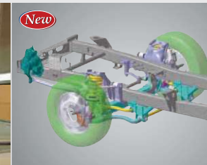
Front Independent Suspension (D4GA Engine only) - Double Wishbone + Coil Spring Type
