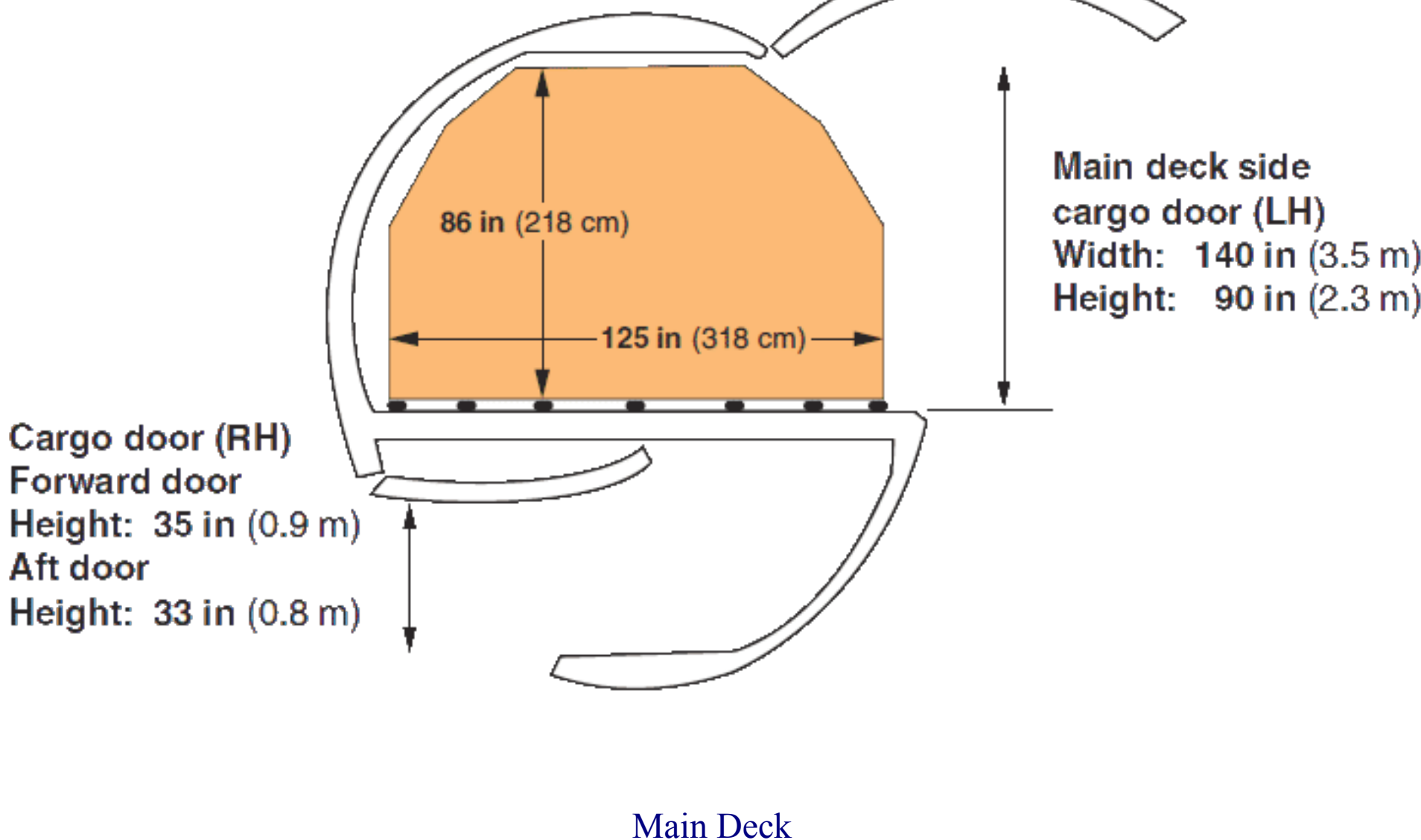
Main Deck
