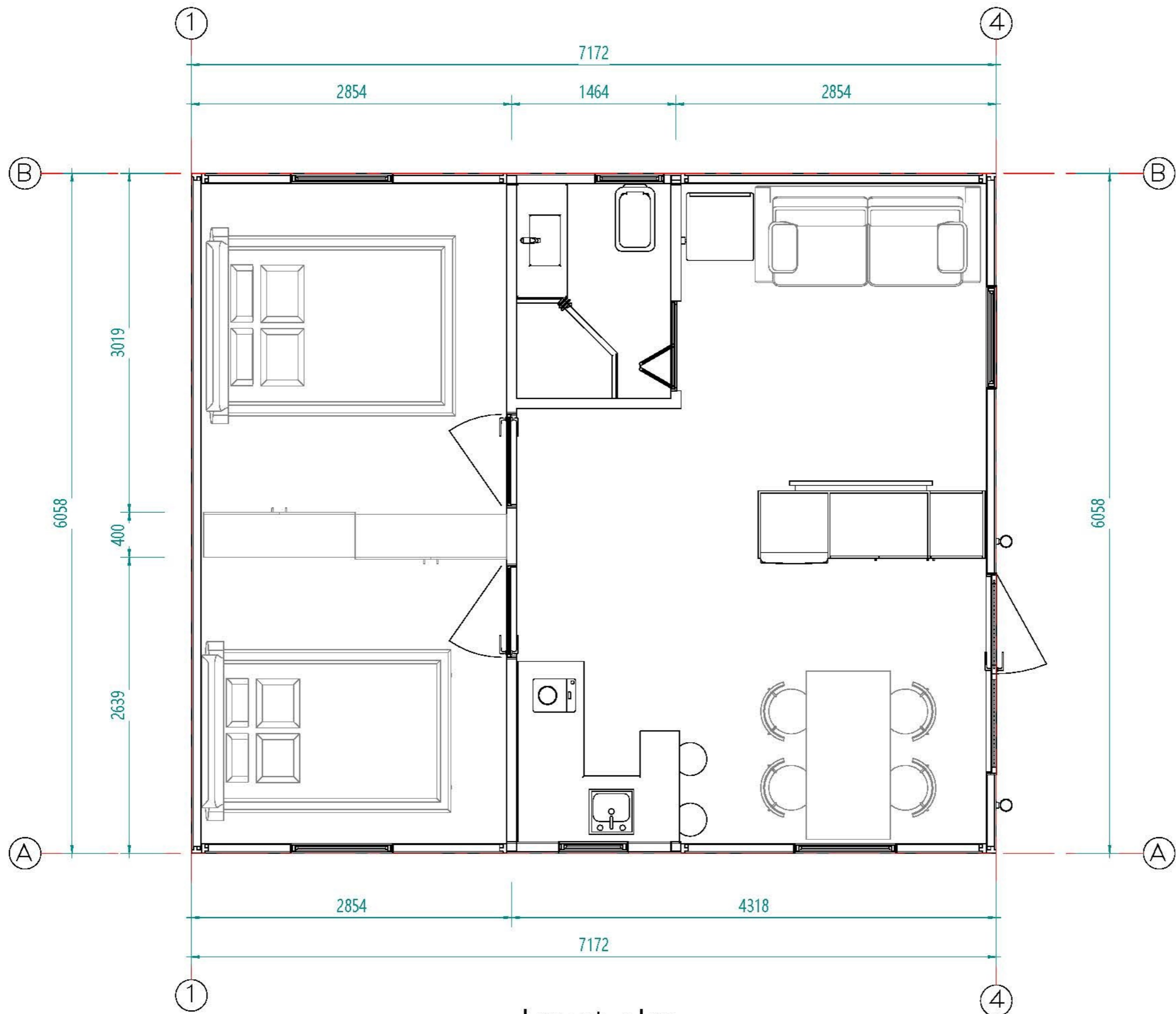
Layout plan
