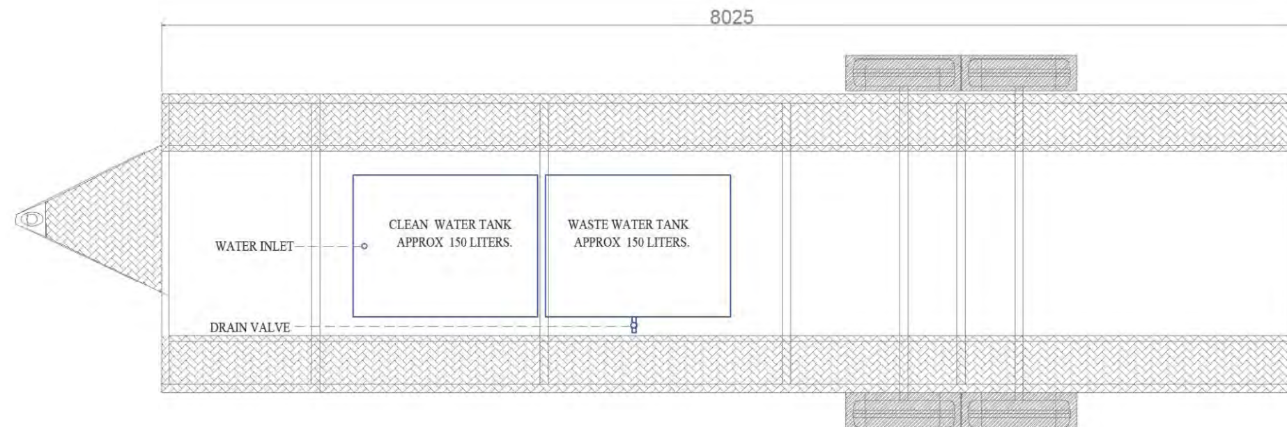
TRAILER PLAN DTL. SCALE: NTS
