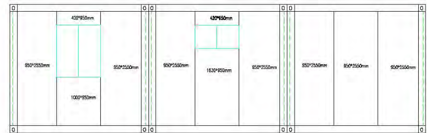
BACK ELEVATION
