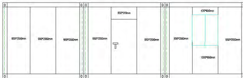
FRONT ELEVATION
