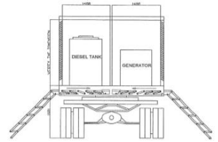
SECTION THRU "A"
