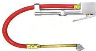
ORIGINAL SERVICE STATION TIRE INFLATOR AND AIR PRESSURE GAUGE, DUAL HEAD CHUCK, 1/4" NPT, 15" RUBBER HOSE 10-160 PSI
