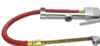
ORIGINAL SERVICE STATION TIRE INFLATOR AND AIR PRESSURE GAUGE, DUAL HEAD CHUCK, 15" RUBBER HOSE, 1/4" NPT 10-160 PSI 1 UNIT
