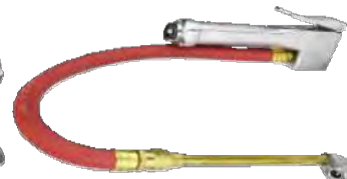
BAYONET TIRE INFLATOR AND AIR PRESSURE GAUGE, DUAL TRUCK TIRE AIR CHUCK, 1/4" NPT, 15" RUBBER HOSE 10-120 PSI 1 UNIT
