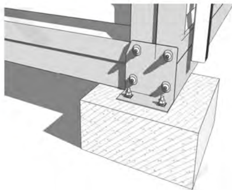
Block foundation
