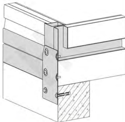
Strip foundation
