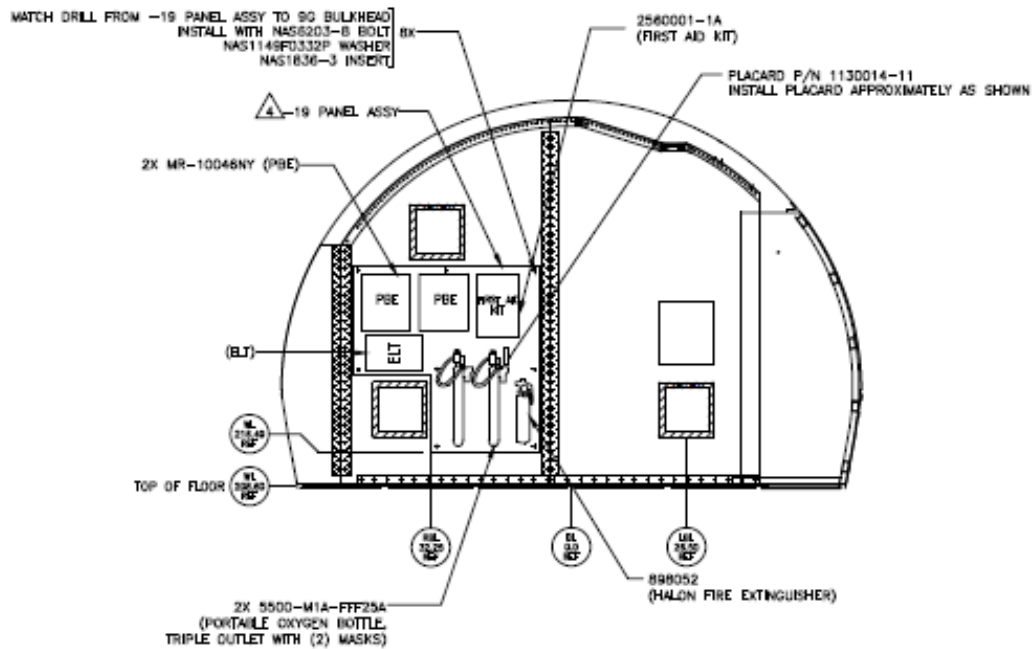
VIEW A-A VIEW LOOKING AFT ROTATED 90° CCW
