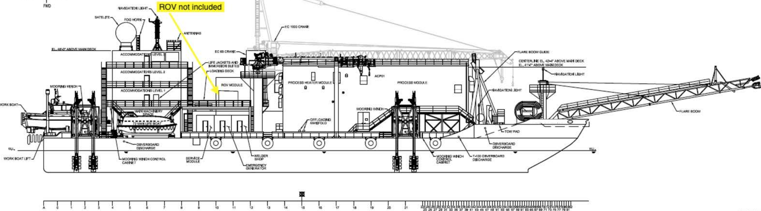
STARBOARD ELEVATION
