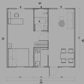
-floor plan-
