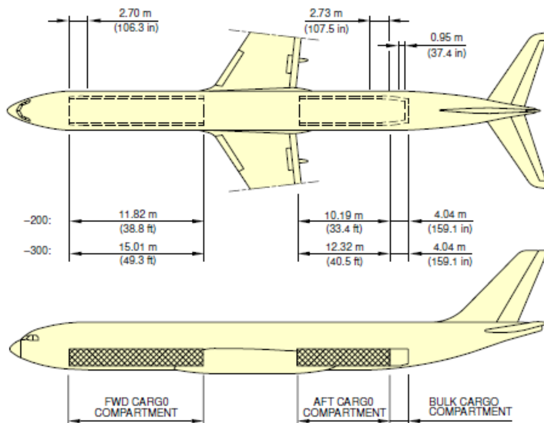
Lower Deck Cargo Compartments FIGURE-2-6-1-991-003-A01
