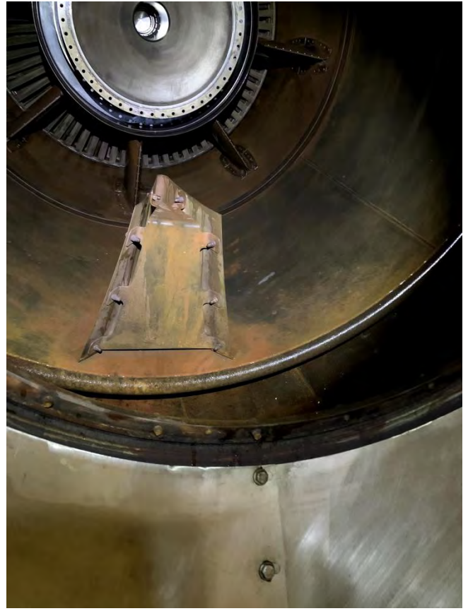
Exhaust
