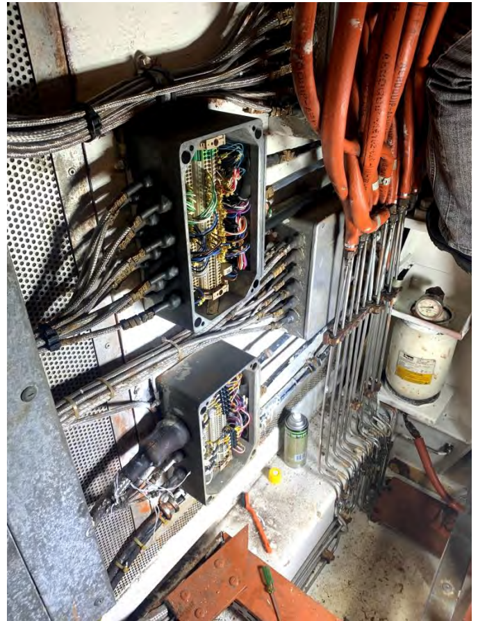
Transducers Boxs
