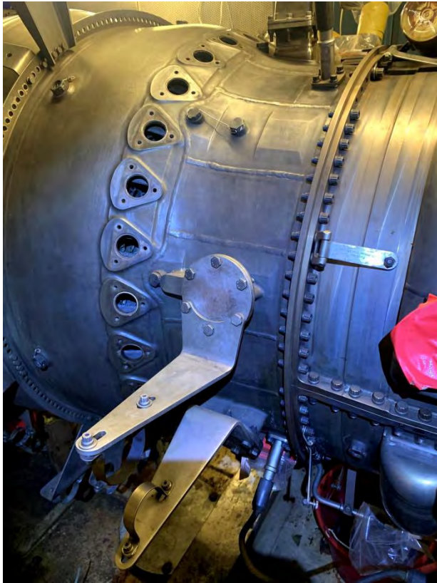
Fuel nozzle clean and Serial Number
