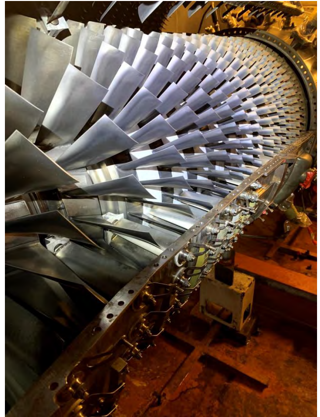
Open Compressor case
