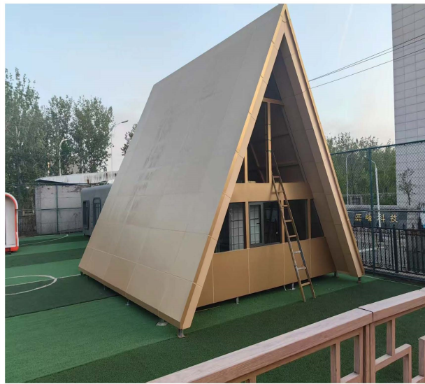
TRIANGULAR HOUSE LAYOUT : 7000mm*5000mm*6000mm with loft
